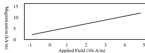
Fig. 1. Magnetization as a function of applied field. Note how the caption is centered in the column.
